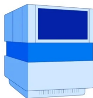
Sequencing
